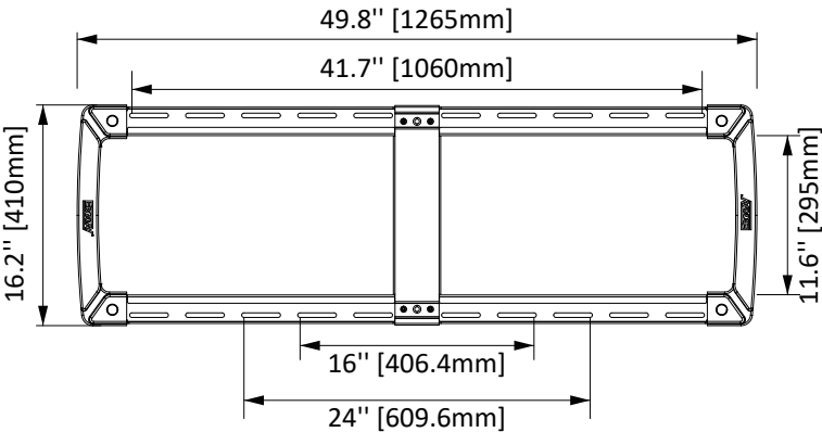
WALL PLATE
