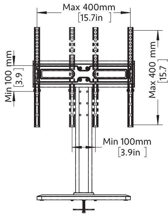
TV INTERFACE
