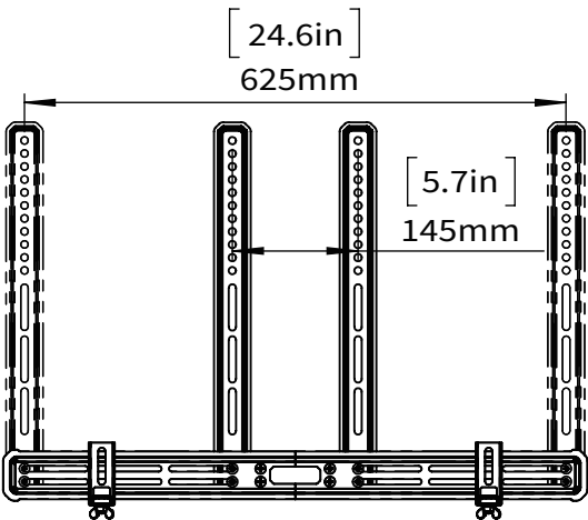
TV INTERFACE
