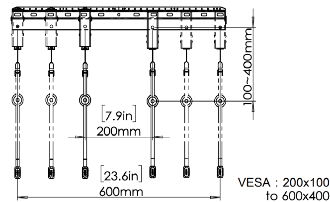
TV INTERFACE
