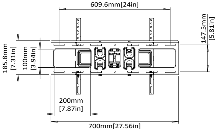
WALL PLATE
