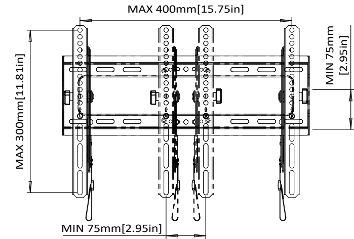
TV INTERFACE
