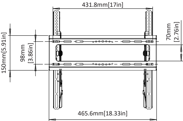
WALL PLATE
