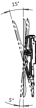
SIDE VIEW - TILTING
