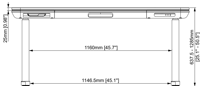
FRONT VIEW
