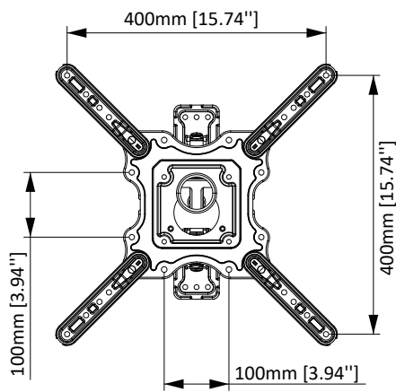
TV INTERFACE
