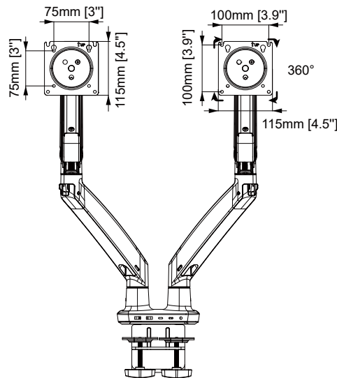
MONITOR INTERFACE
