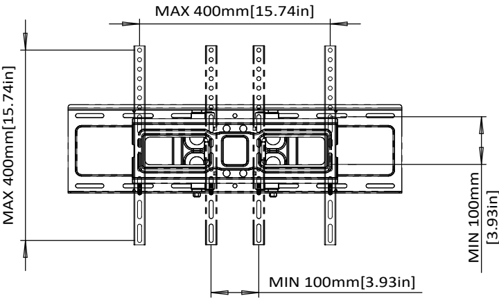
TV INTERFACE
