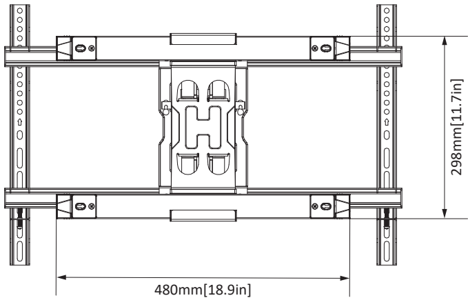
WALL PLATE
