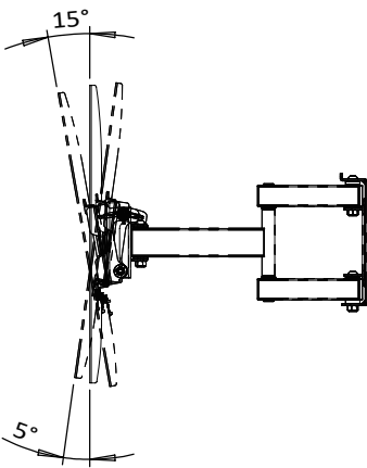
SIDE VIEW - TILTING
