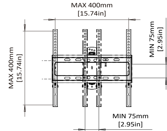
TV INTERFACE
