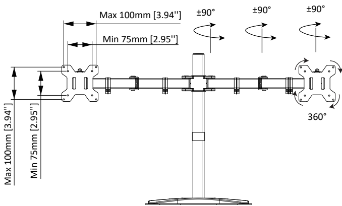
MONITOR INTERFACE
