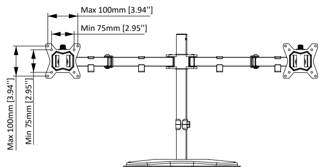
MONITOR INTERFACE
