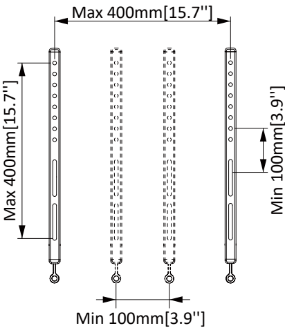
TV INTERFACE
