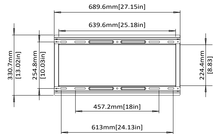
WALL PLATE
