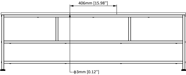
BACK VIEW
