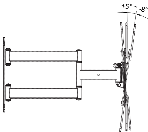
SIDE VIEW - TILTING
