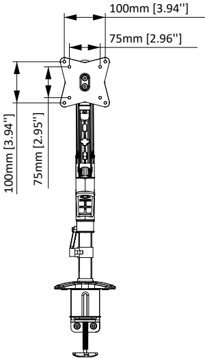
MONITOR INTERFACE
