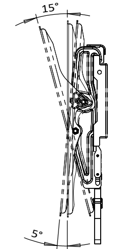
SIDE VIEW - TILTING
