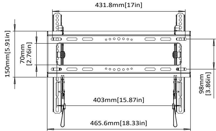
WALL PLATE
