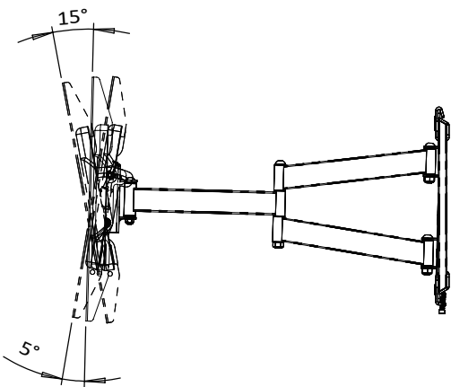
SIDE VIEW - TILTING
