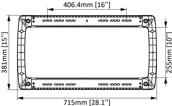
WALL PLATE
