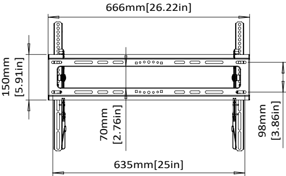
WALL PLATE
