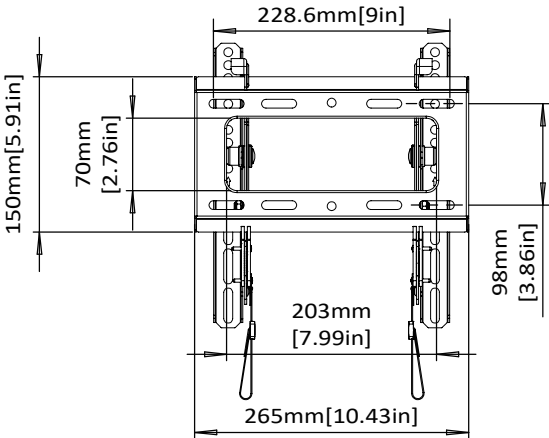
WALL PLATE
