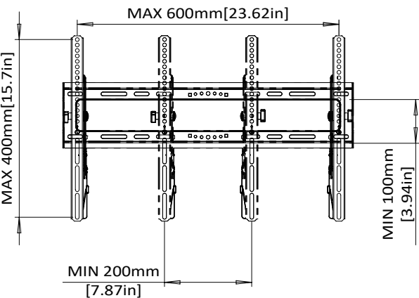
TV INTERFACE
