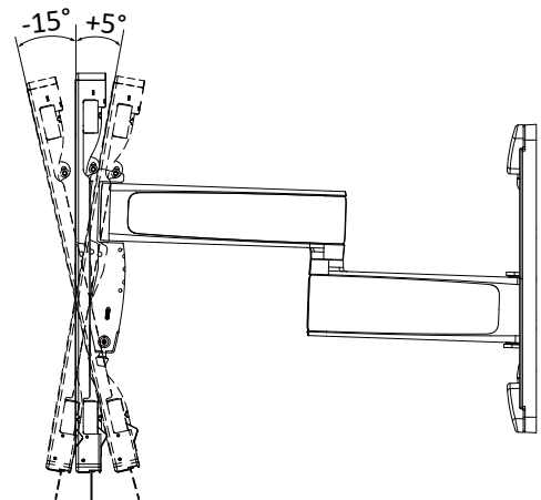
SIDE VIEW - TILTING
