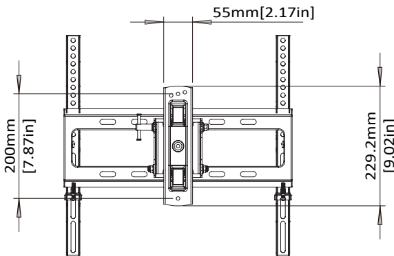
WALL PLATE
