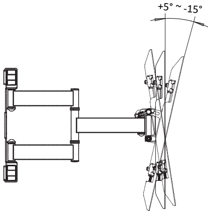
SIDE VIEW - TILTING
