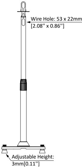
BACK VIEW
