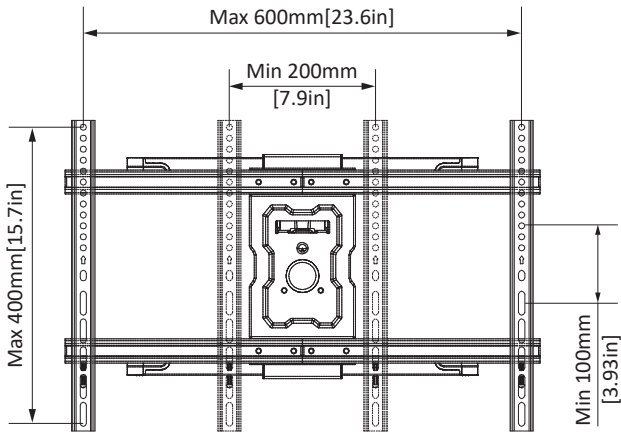
TV INTERFACE
