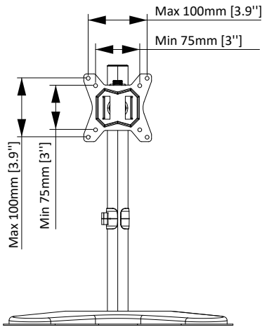
MONITOR INTERFACE
