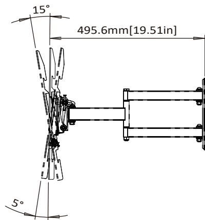
SIDE VIEW - TILTING
