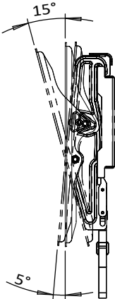
SIDE VIEW - TILTING
