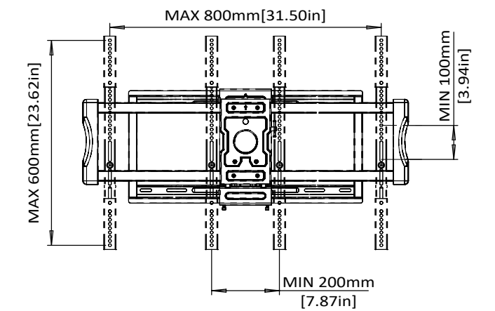
TV INTERFACE
