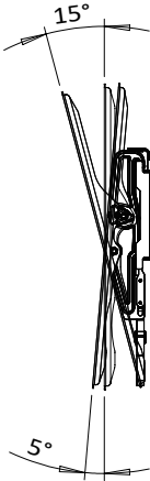
SIDE VIEW - TILTING
