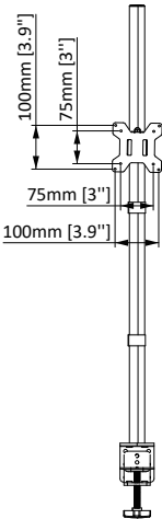
MONITOR INTERFACE
