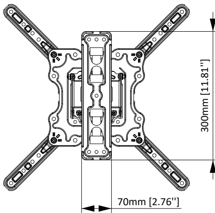
WALL PLATE
