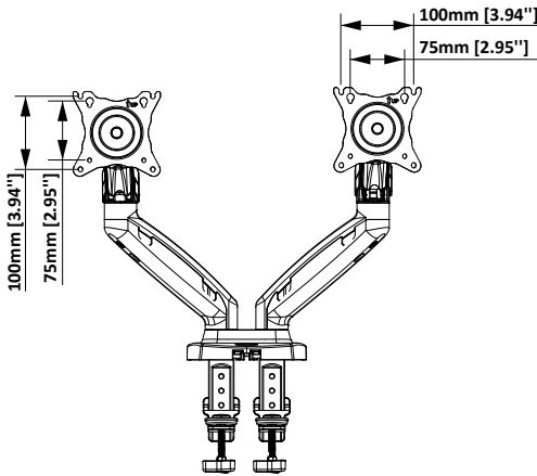
MONITOR INTERFACE
