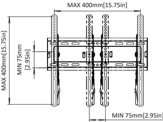
TV INTERFACE
