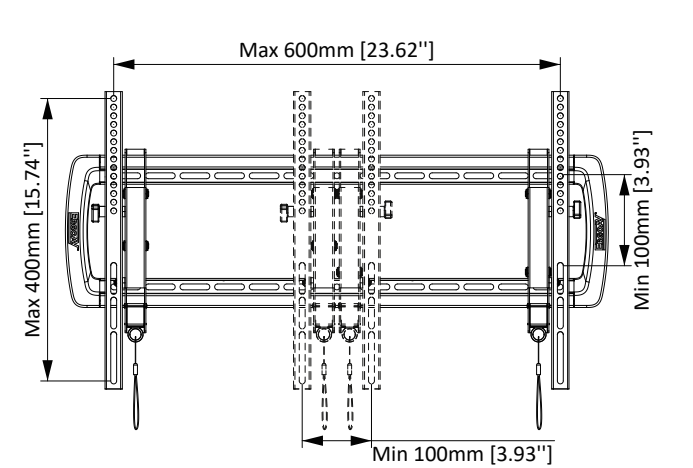
TV INTERFACE
