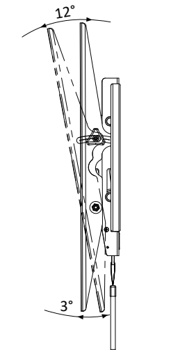
SIDE VIEW - TILTING
