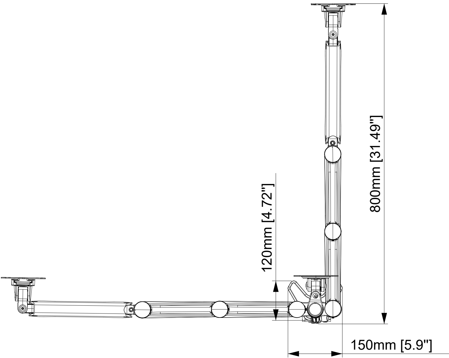
TOP VIEW
