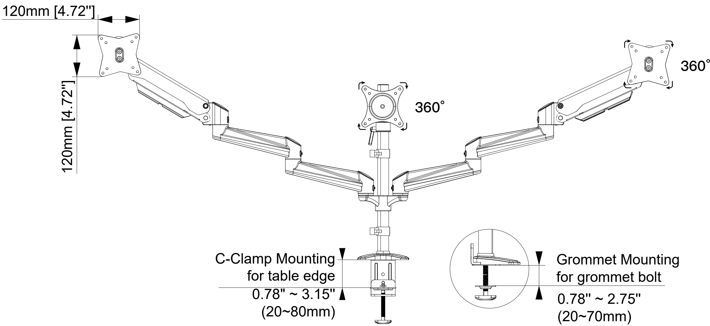
FRONT VIEW
