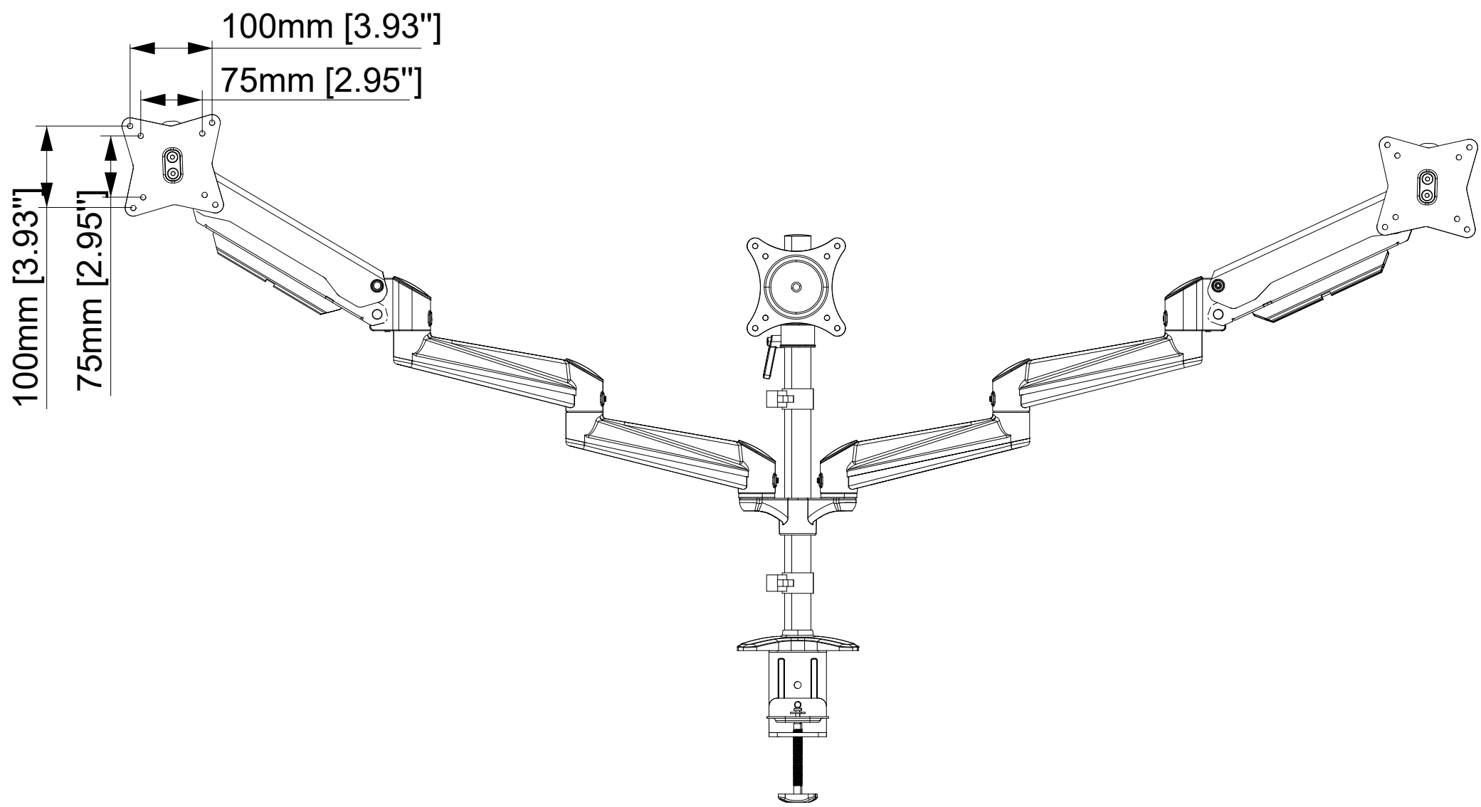
TV INTERFACE
