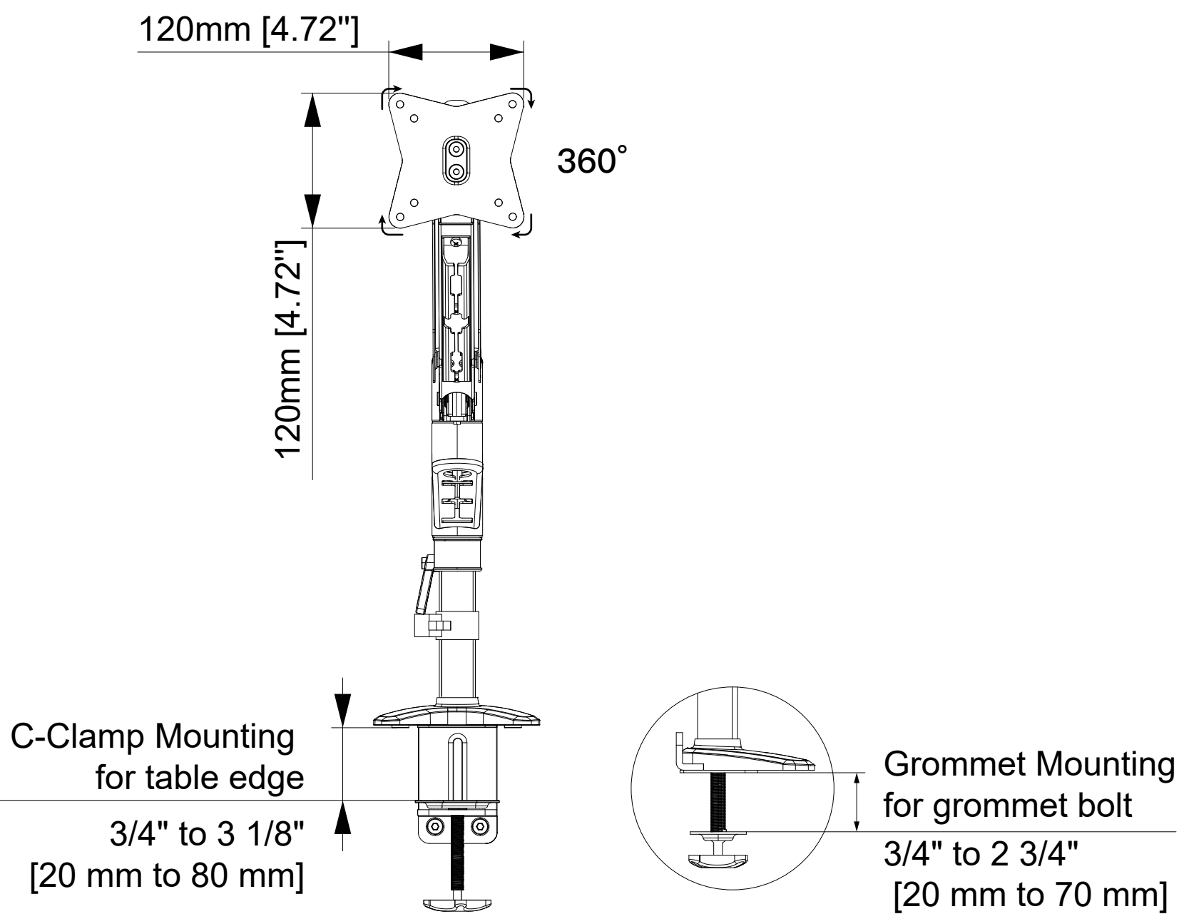
FRONT VIEW
