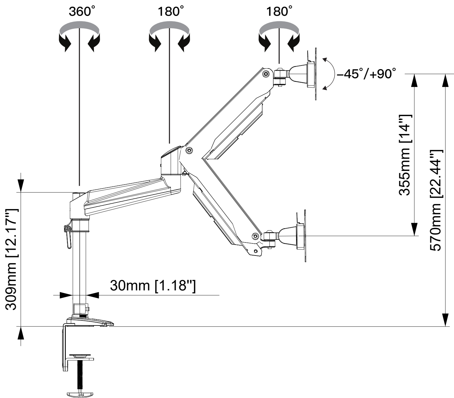
SIDE VIEW
