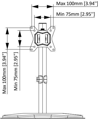
MONITOR INTERFACE
