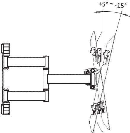
SIDE VIEW - TILTING
