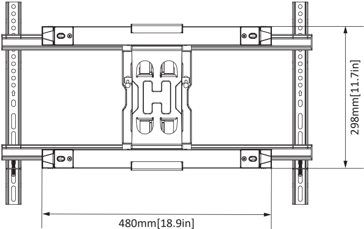
WALL PLATE
