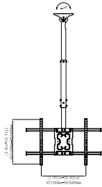
BACK VIEW
