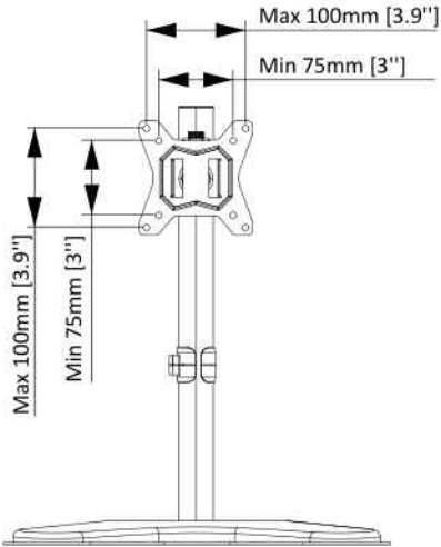
MONITOR INTERFACE
